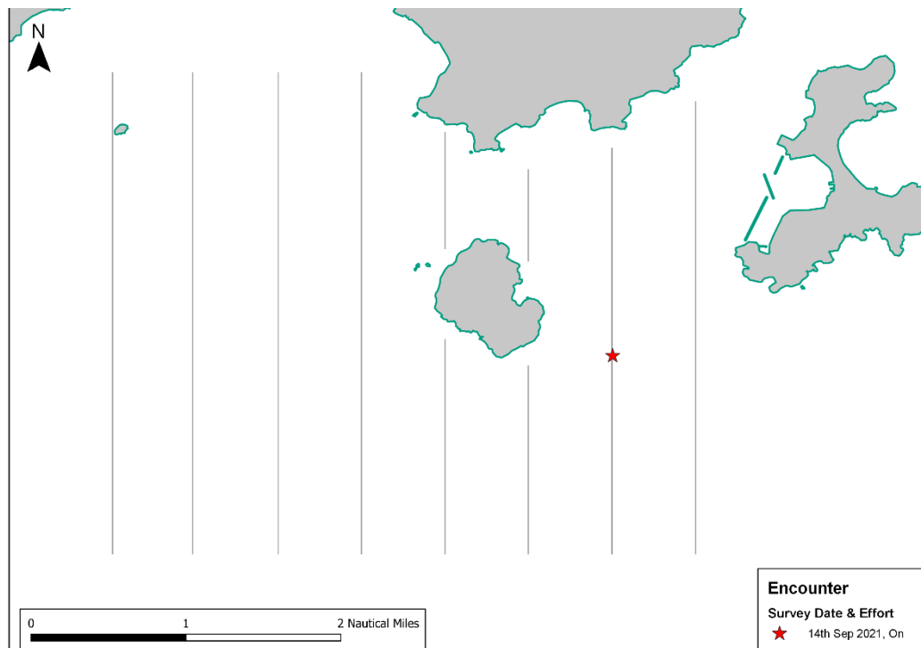
Figure 6.5 Location of sightings recorded during September 2021 Vessel-based Line-transect Survey
